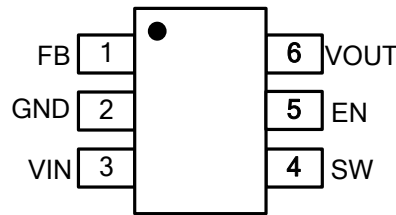
Top View SOT563
