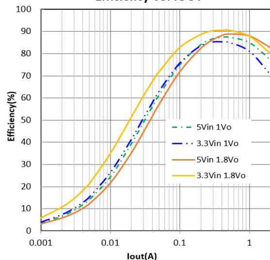
MT8092AGAR Efficiency VS. IOUT
