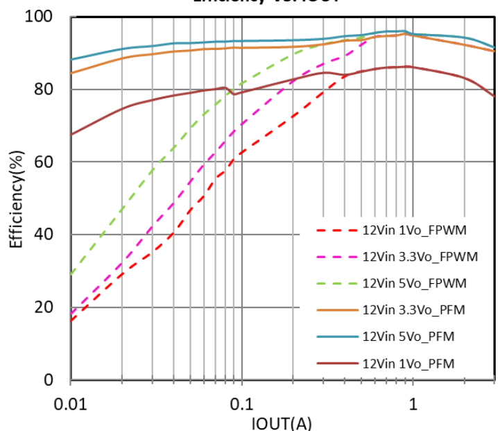
Efficiency VS. IOUT
